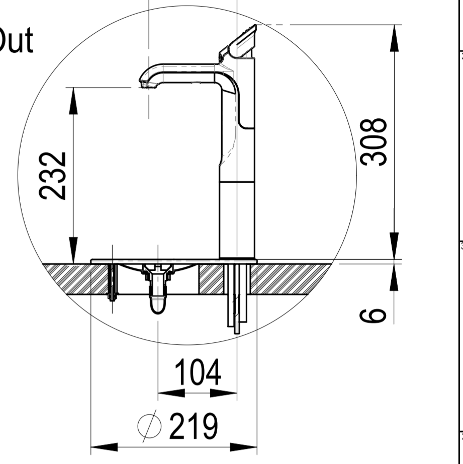
DETAIL FRONT SCALE 1 : 5
